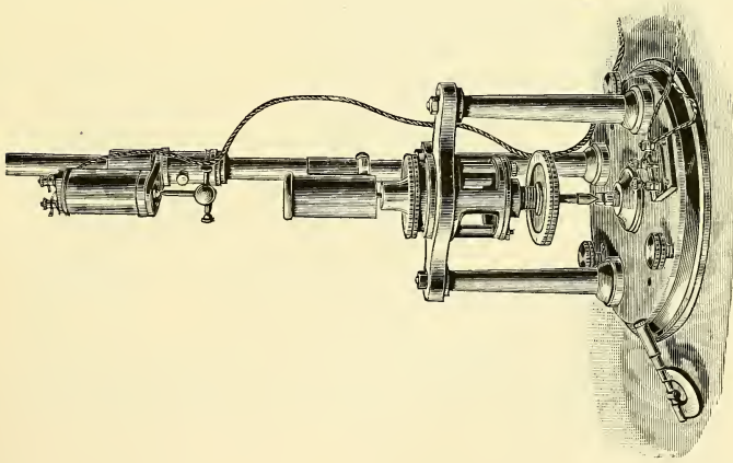
Borland's Cap Tester.
